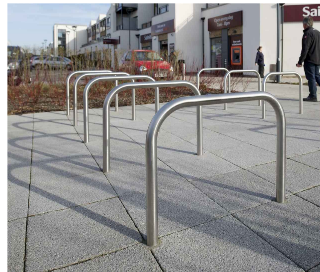
02 TYPICAL SHEFFIELD STAND DETAIL SCALE: 1:10 @A1
